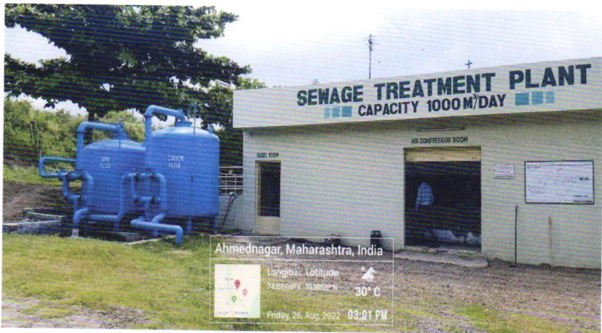
Carbon and Sand Filter
